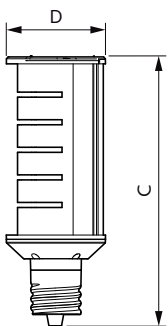
Wallpack LED 40W EX39 850 CL
