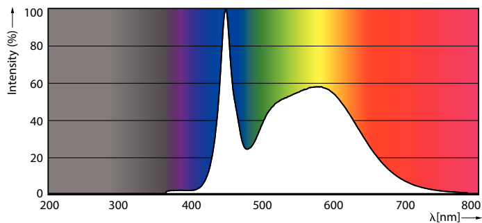
LEDTForce 40W WallPack EX39 850
