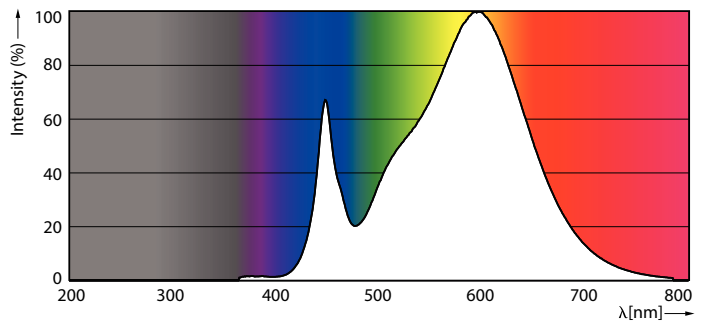
LEDTForce 36W Corncob 830
