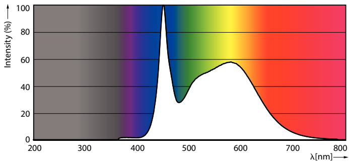
LEDForce 36W Corncob 850
