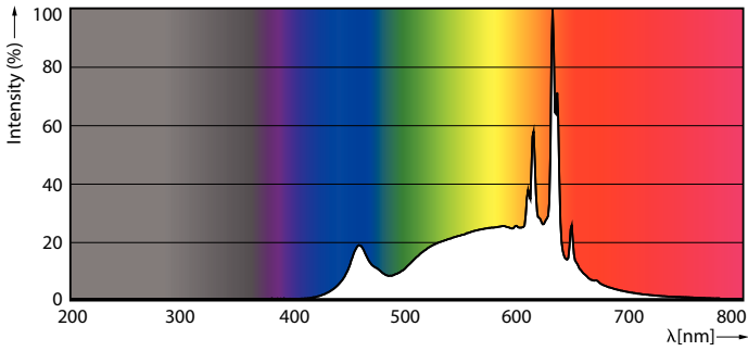
LEDbulb 16W A21 GU24 930 FR
