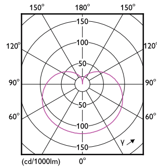
LEDbulb A21 GU24 1600lm FR
