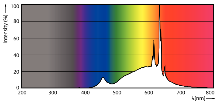
LEDbulb 65W E26 BR40 927 Frosted
