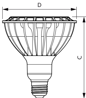
PAR38 120V 32-W 2800lm 15D 3000K E26 D
