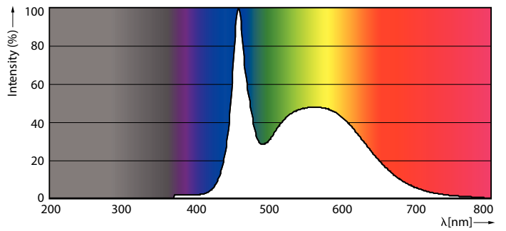
LEDbulb 20W A30 E26 865 15D ND
