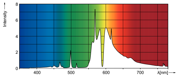
LDPO_SONHORT_0001-Spectral power distribution Colour
