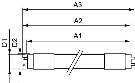
Smart TypeB 120-277 14.5W 2000lm 3500K
