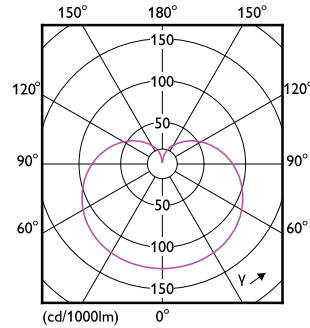
LEDbulb A19 16W E26 1600lm 930 FR
