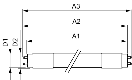
14.5T8/MAS/48-830/MF20/P 10/1
