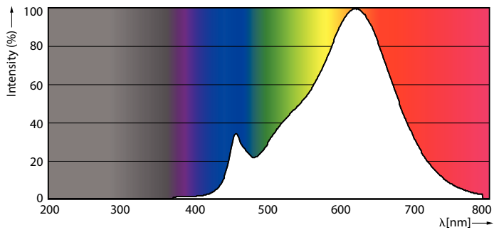
LEDbulb CL,FR 927
