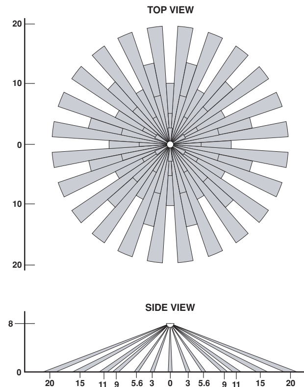
Figure 2 (Cat. No. LRM225000) Field-of-View Ranges
